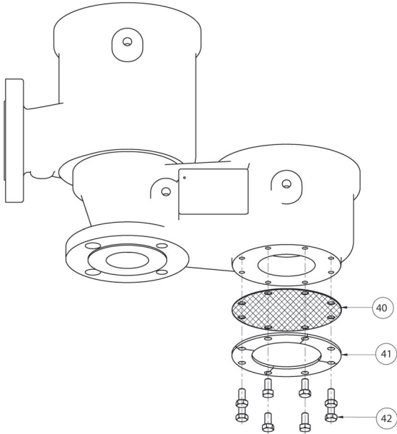
Figure 10 - Flame Screen
