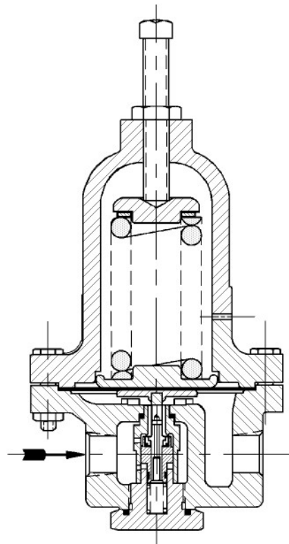
Figure 3: Model HP Cut-away
