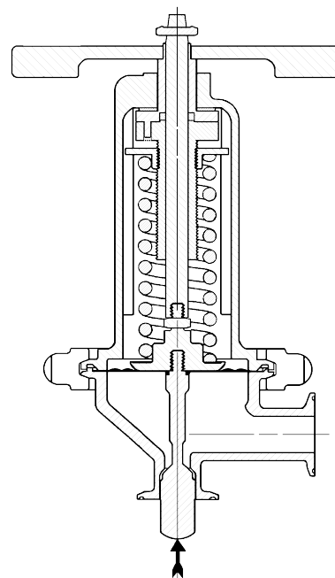
1" Size Investment Cast Body Metal Seat
