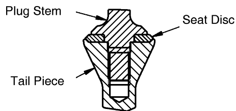
Composition Seat (Not available for Investment Cast Body)
